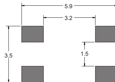
Recommended layout for solder pads
